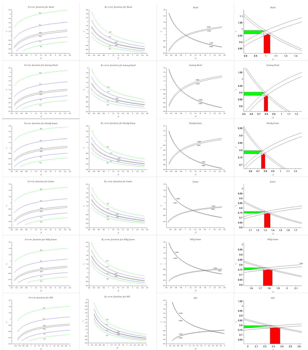
FIGURE 2 S and K_s error functions contours for 0.1 initial degree of saturation, (the green, blue and black lines represent respectively error value of 0.2, 0.1 and 0.01) and error functions intersection for S and K_s and for 0.005 error value.
